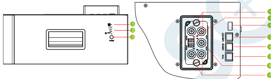
Fig 1.2: Introduction to the battery operation panel
