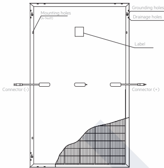
Figure 2: Example of product technical drawings
