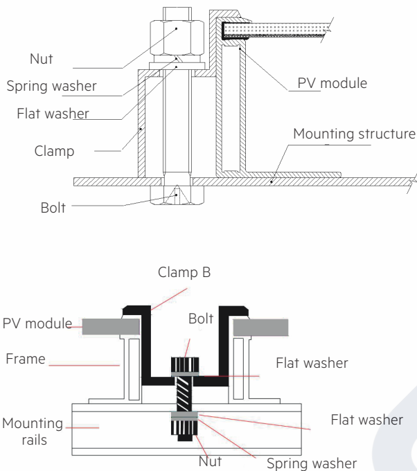
Figure 4: Examples of clamping
